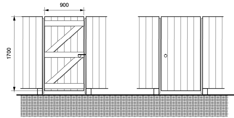
Rear Elevation Timber garden gate
