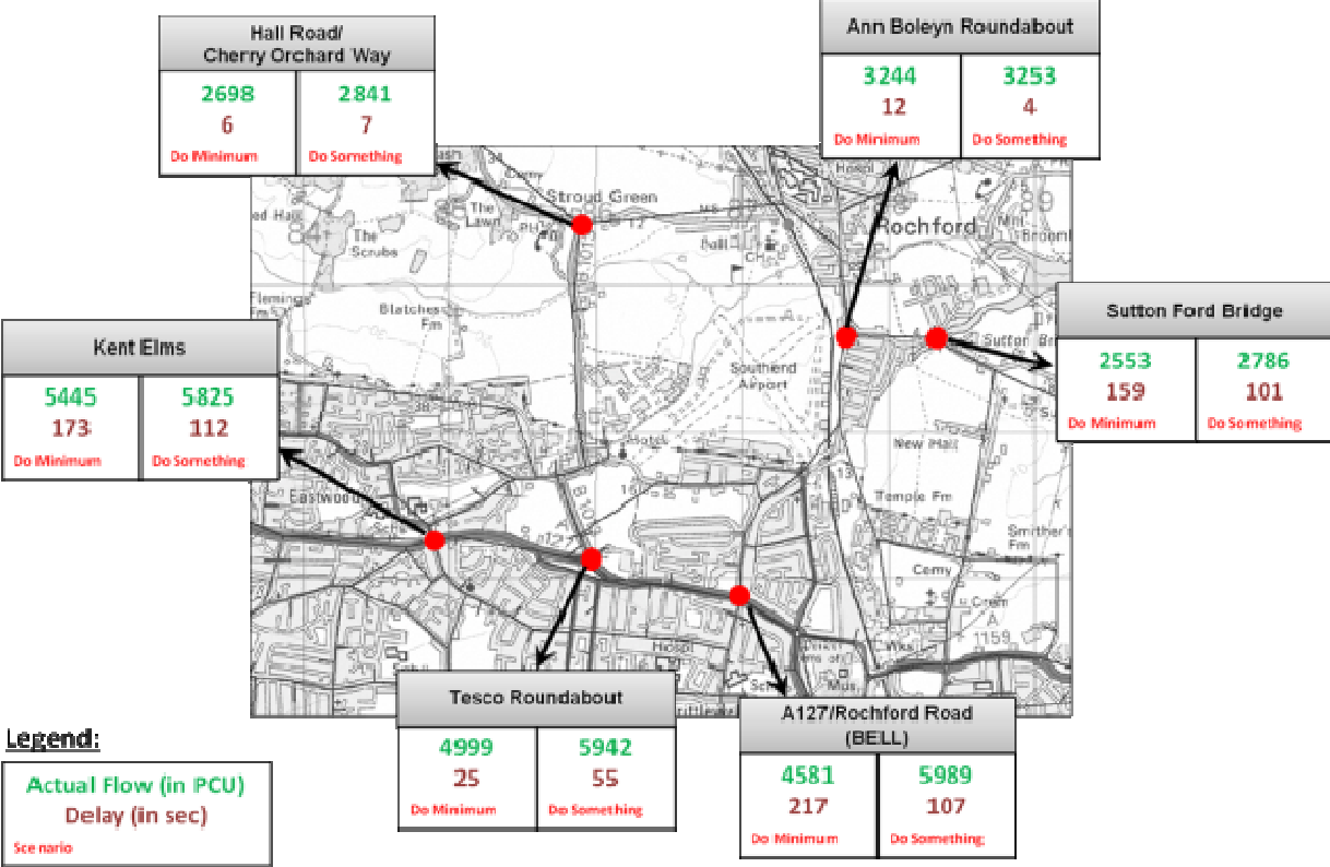
Figure 14. Rochford and A127 Junctions (average delay seconds) AM Peak 2021
