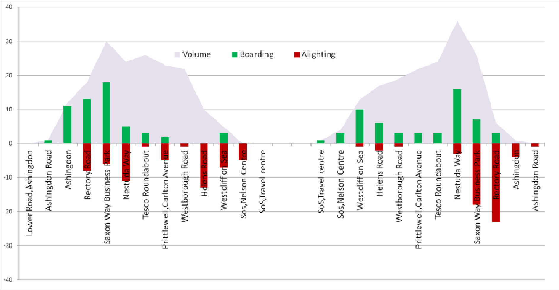
Figure 24. Route C Boarding and Alighting AM Peak hour 2021
