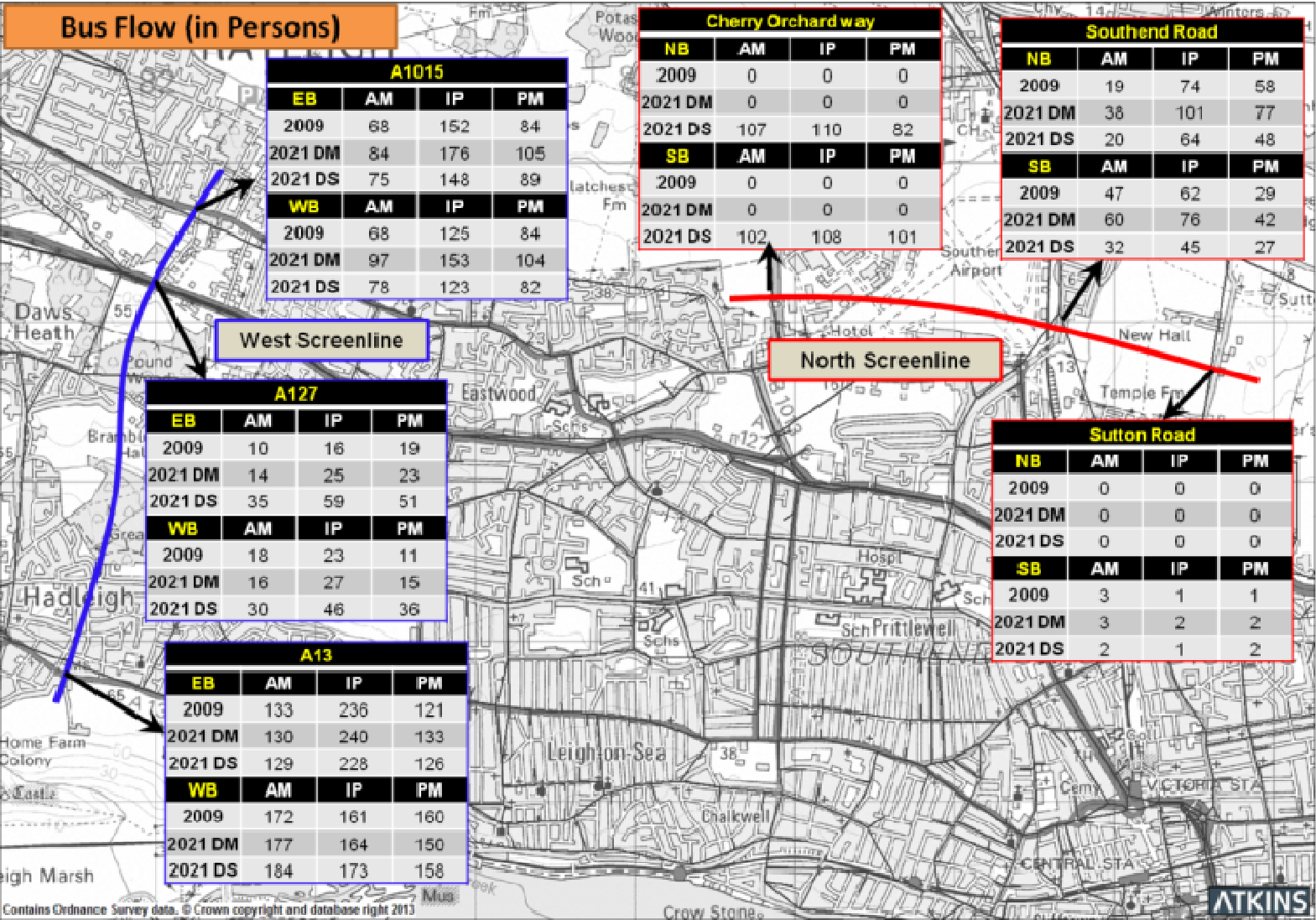
Figure 18. Screenline Flows- Bus Flows (in Persons) 2021
