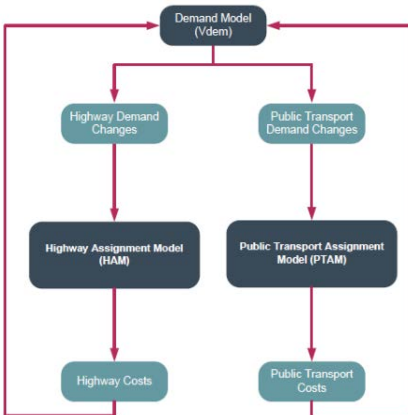
Figure 2. Southend Forecast Model Structure
