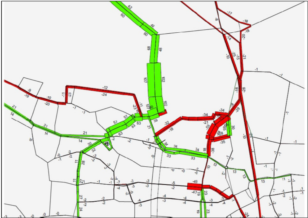
Figure 15. Public Transport Passengers Flow Difference (Do Something – Do Minimum) AM Peak 2021
