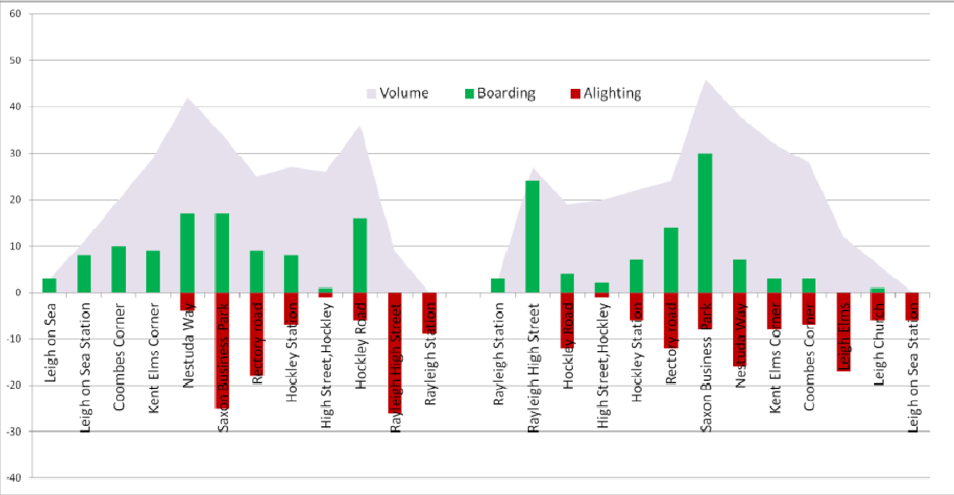
Figure 22. Route A Boarding and Alighting AM Peak hour 2021
