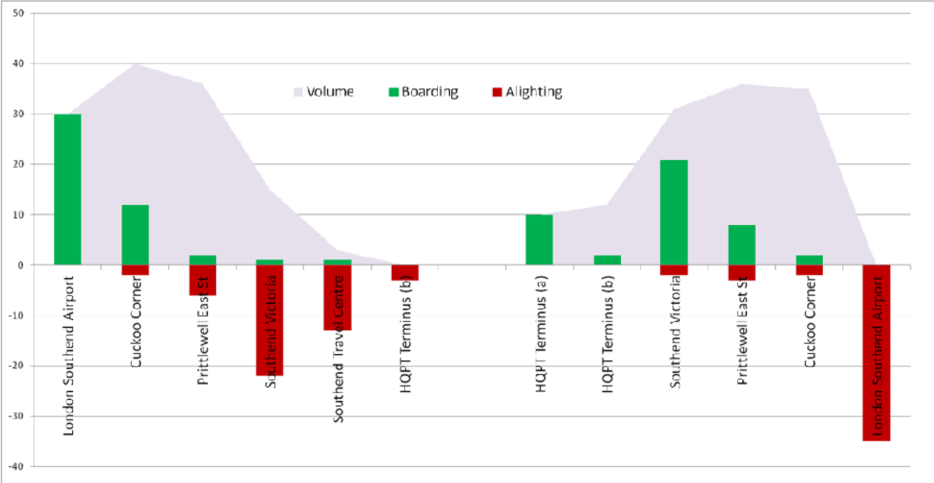
Figure 20. HQPT Boarding and Alighting AM Peak hour 2021
