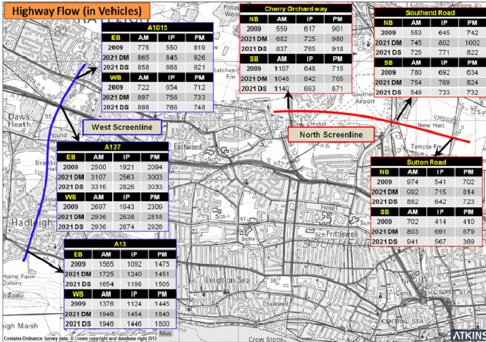
Figure 17. Screenline Flows- Highway Flows (in Vehicles) 2021
