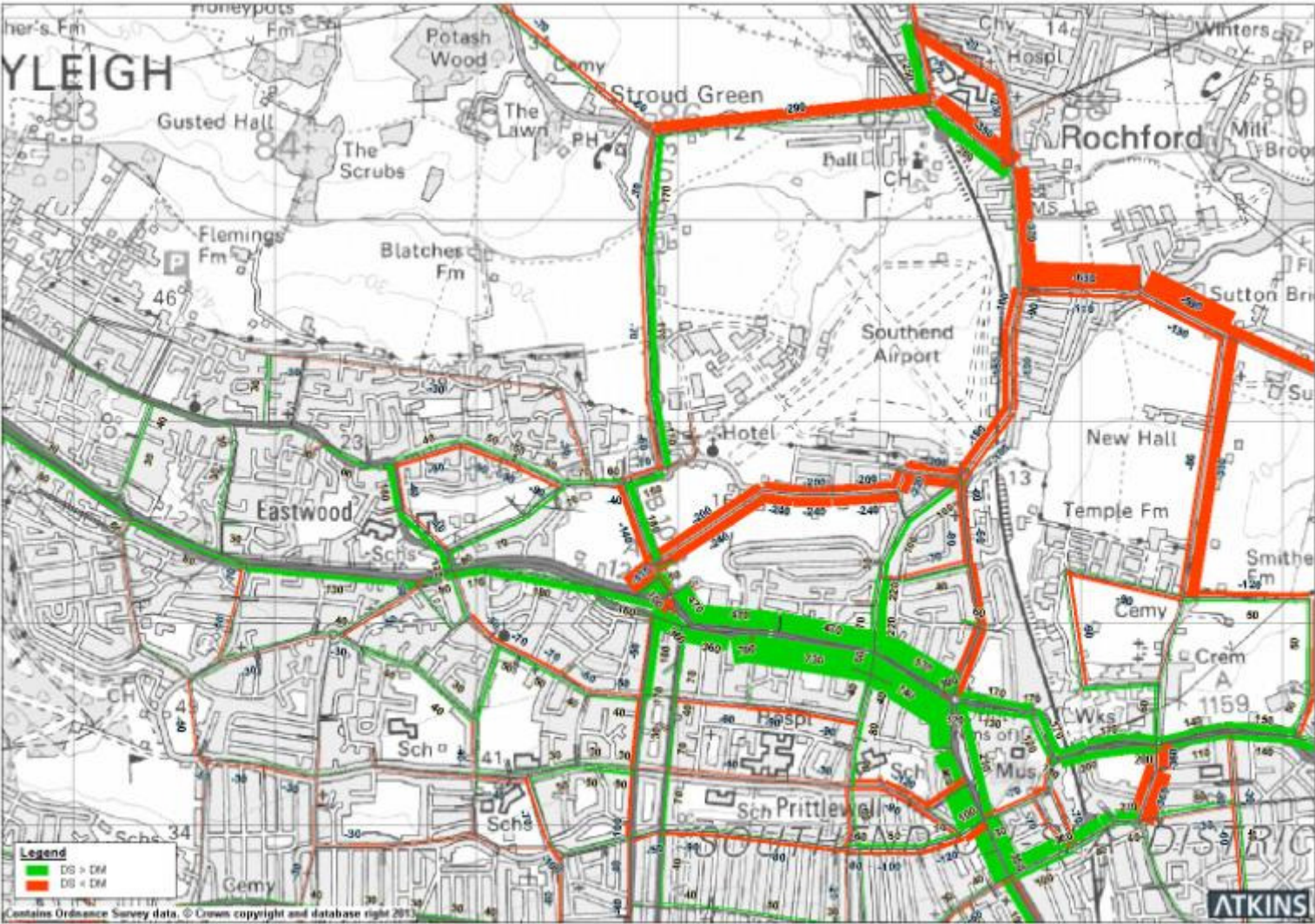
Figure 11. Highway Flow Difference (Do Something – Do Minimum) PM Peak 2021
