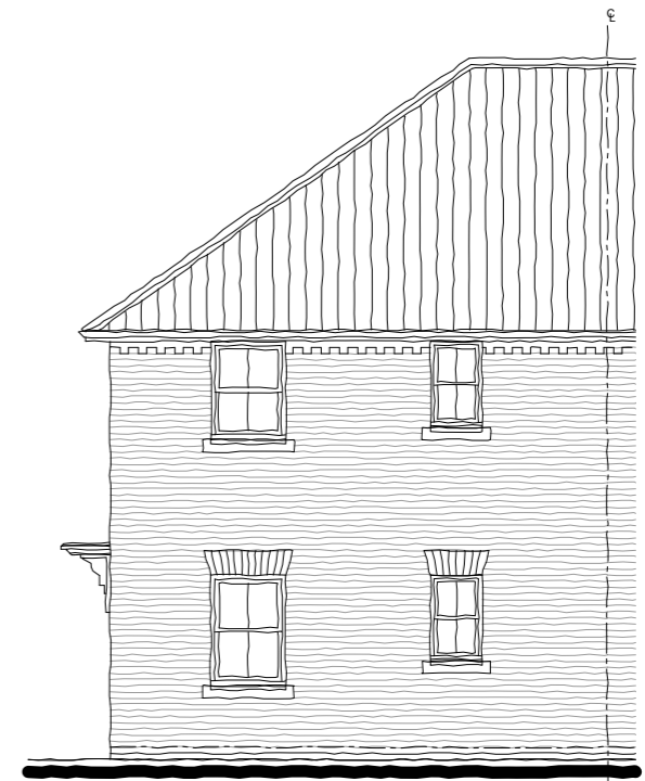
Rear Elevation 2
