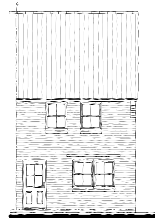
Rear Elevation
