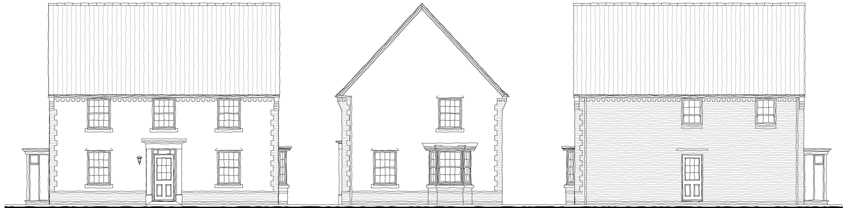
Front Elevation
