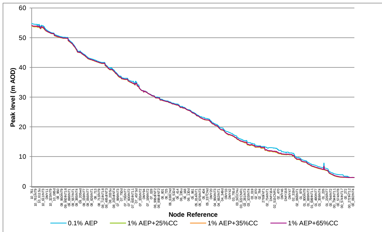
Figure C2 - Prittle Brook Peak Flood Level Long Section
